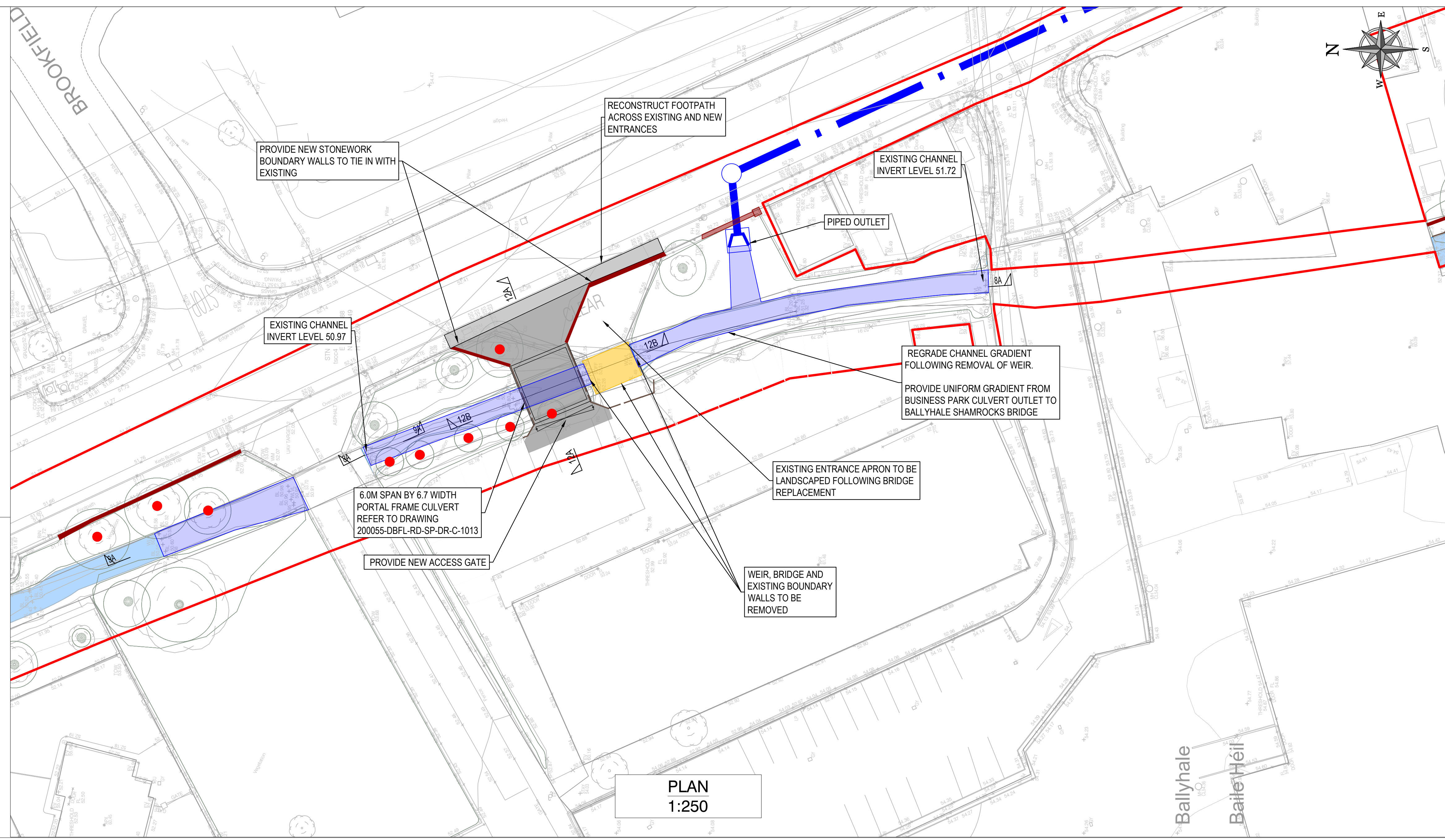
EXISTING WEIR AND BRIDGE TO BE REMOVED
