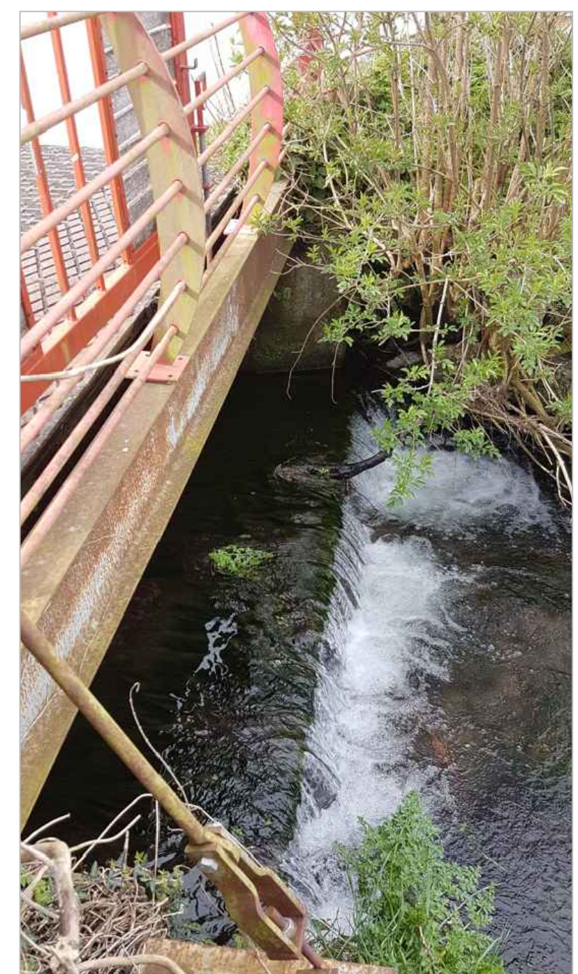
EXISTING WEIR AND BRIDGE TO BE REMOVED
